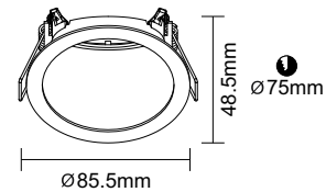
● 2448-28CR Material: Aluminum / Iron Light Source: MR16 Light Source Replaceable IP20 / Class 1/CE Powder Injection Black / White
