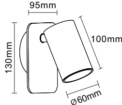
● 2433-24AA Material: Aluminum Light Source: GU10 Wire: 2/3/4 Light Source Replaceable IP20 / Class 1/CE Anodized Silver / Powder Injection Black / White
