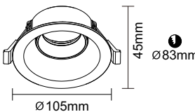
● 2447-23CR Material: Aluminum / Iron Light Source: MR16 Light Source Replaceable IP20 / Class 1/CE Powder Injection Black / White
