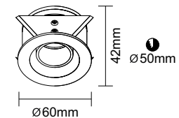
● 2448-42DR Material: Aluminum / Iron Light Source: MR11 Light Source Replaceable IP20 / Class 1/CE Powder Injection Black / White
