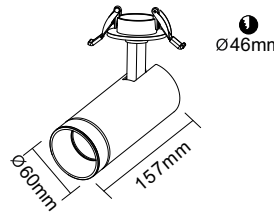
● 2434-14CA Material: Aluminum Light Source: GU10 Wire: 2/3/4 Light Source Replaceable IP20 / Class 1/CE Anodized Silver / Powder Injection Black / White
