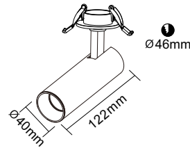
● 2434-11CA Material: Aluminum Light Source: GU10 Wire: 2/3/4 Light Source Replaceable IP20 / Class 1/CE Anodized Silver / Powder Injection Black / White
