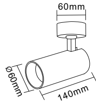
● 2433-32BA Material: Aluminum Light Source: AR70 Wire: 2/3/4 Light Source Replaceable IP20 / Class 1/CE Anodized Silver / Powder Injection Black / White
