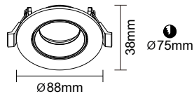
● 2447-13CR Material: Aluminum / Iron Light Source: MR16 Light Source Replaceable IP20 / Class 1/CE Powder Injection Black / White
