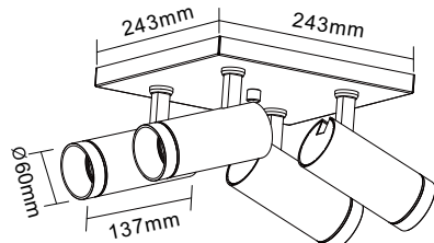
2432-31CD Material: Aluminum Light Source: GU10 Wire: 2/3/4 Light Source Replaceable IP20 / Class 1/CE Anodized Silver / Powder Injection Black / White
