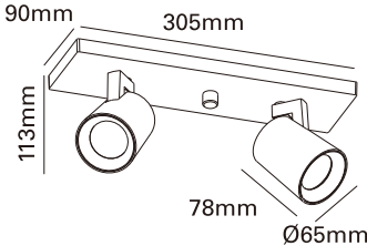
2431-32CB Material: Aluminum Light Source: GU10 Wire: 2/3/4 Light Source Replaceable IP20 / Class 1/CE Anodized Silver / Powder Injection Black / White
