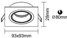
● 2447-T209 / T203 / T223 Material: Aluminum / Iron Light Source: MR16 Light Source Replaceable IP20 / Class 1/CE Powder Injection Black / White / Nikkel
