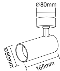
● 2433-32BA Material: Aluminum Light Source: AR70 Wire: 2/3/4 Light Source Replaceable IP20 / Class 1/CE Anodized Silver / Powder Injection Black / White
