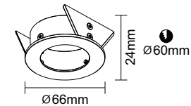
● 2448-14CR Material: Aluminum / Iron Light Source: MR16 Light Source Replaceable IP20 / Class 1/CE Powder Injection Black / White
