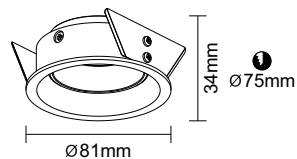
● 2447-26CR Material: Aluminum / Iron Light Source: MR16 Light Source Replaceable IP20 / Class 1/CE Powder Injection Black / White
