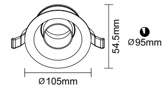
● 2448-42CR Material: Aluminum / Iron Light Source: MR16 Light Source Replaceable IP20 / Class 1/CE Powder Injection Black / White
