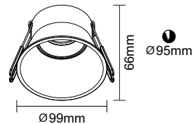
● 2447-24CR Material: Aluminum / Iron Light Source: MR16 Light Source Replaceable IP20 / Class 1/CE Powder Injection Black / White
