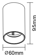
● 2433-15AR Material: Aluminum Light Source: GU10 Wire: 2/3/4 Light Source Replaceable IP20 / Class 1/CE Anodized Silver / Powder Injection Black / White
