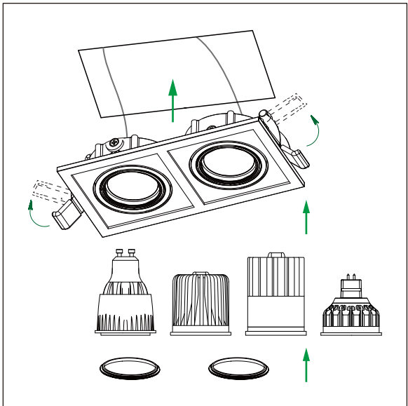
● 2440-32CA / 2440-32CB / 2440-32CC Material: Aluminum / Iron Light Source: MR16 Installation: Frame Light Source Replaceable IP20 / Class 1/CE Powder Injection Black / White
