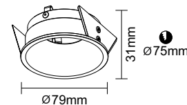
● 2448-25CR Material: Aluminum / Iron Light Source: MR16 Light Source Replaceable IP20 / Class 1/CE Powder Injection Black / White
