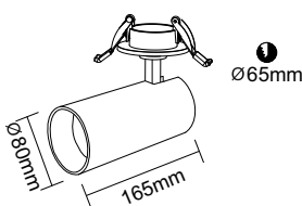
● 2434-11BA Material: Aluminum Light Source: AR70 Wire: 2/3/4 Light Source Replaceable IP20 / Class 1/CE Anodized Silver / Powder Injection Black / White
