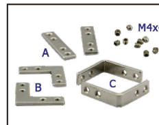
Connector A) Direct B) 90° inside C) 90° outside
