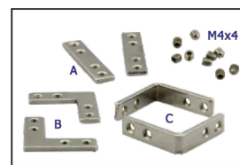
Connector A) Direct B) 90° inside C) 90° outside
