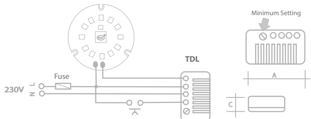
High Voltage LED Module
